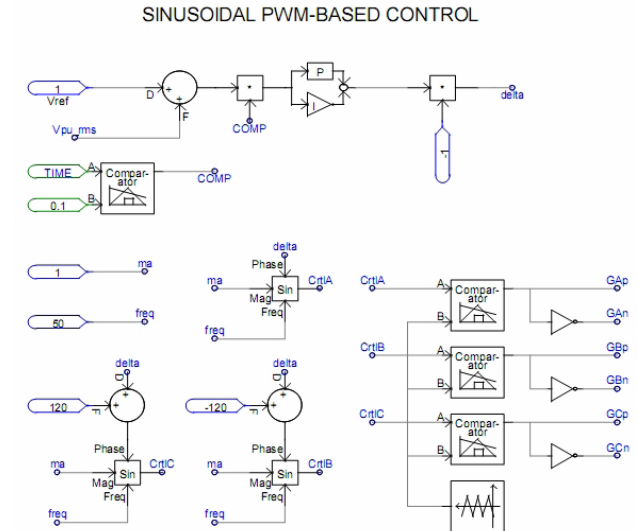
Fig.1. PWM based control scheme
