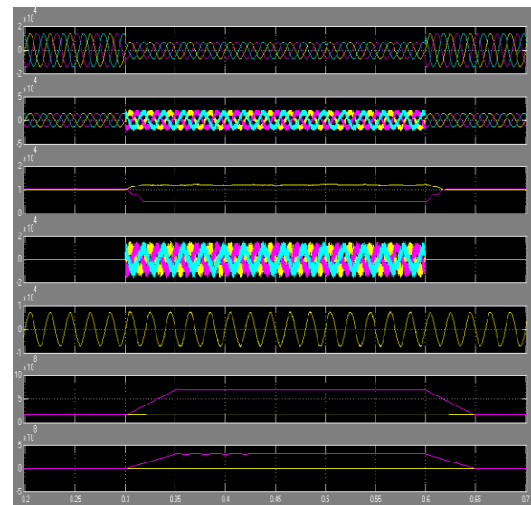
Fig. 4 Simulation results- Mitigation of voltage sag (impulsive) Using IUPQC
