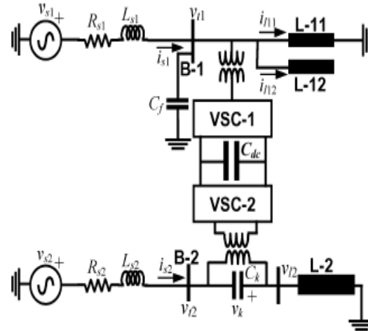
Fig.2. Typical IUPQC connected in a distribution system
