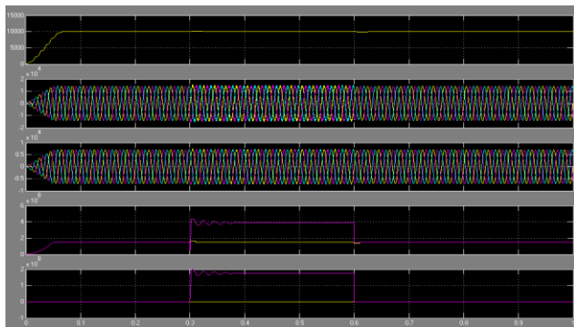
Fig.3 Simulation results – Comparison of Waveforms for a voltage sag of 81% with and without UPQC
