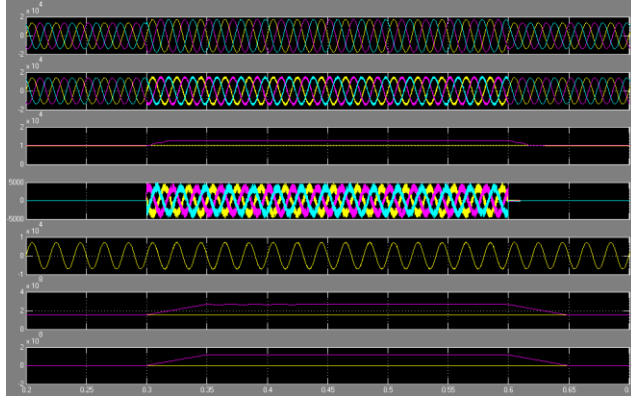
Fig.5. Simulation results- Mitigation of a voltage swell (momentary)
